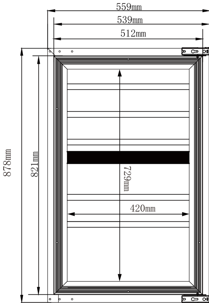
Front View
